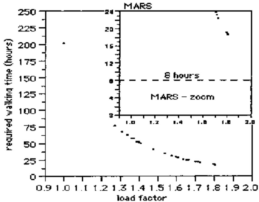
Figure 9. Required walking time on Mars with various load factors to
