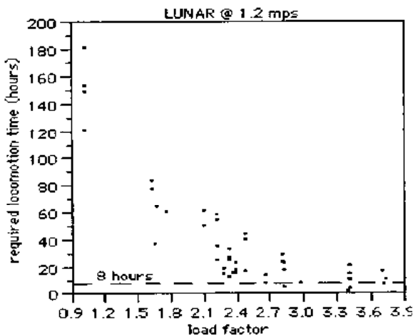
Figure 13. Predicted locomotion time required on the moon at 1.2 mps with various load factors to maintain bone mass at the level of amoderately active individual on earth, using equation (#).
